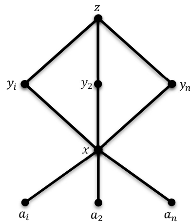
Gambar 4. Jellyfish Graph ( Jf_n )
