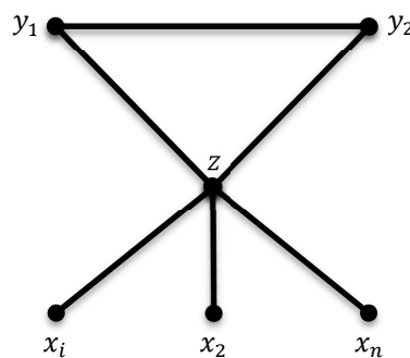
Gambar 3. Squid Graph ( Sq_n )
