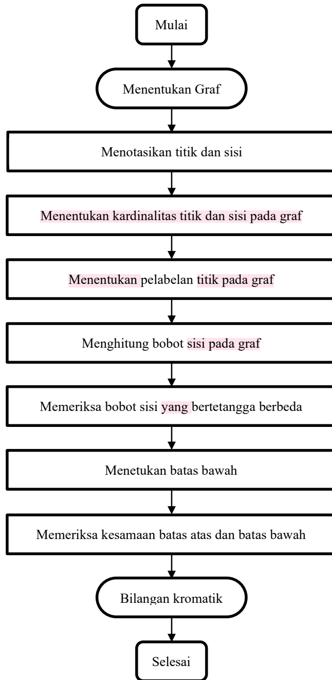
Gambar 1. Alur Penelitian
