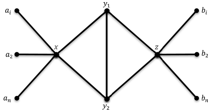
Gambar 2. Crab Graph ( Cr_n )
