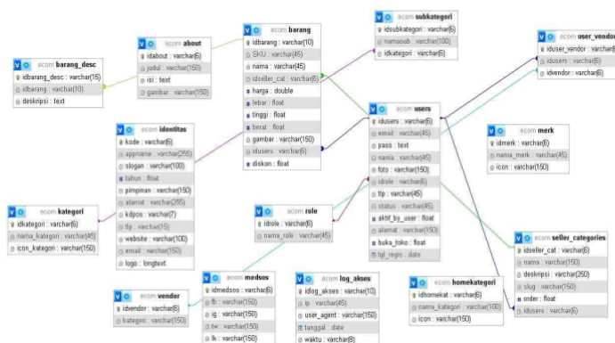
Gambar 7. Class Diagram
