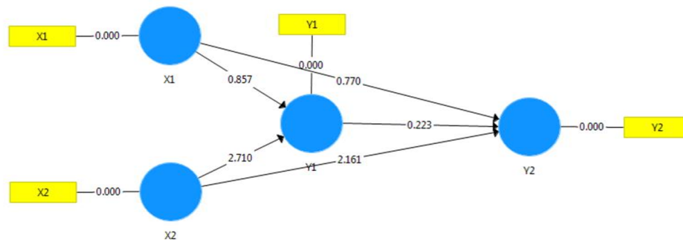
Gambar 2 Hasil Uji Model Struktural PLS
