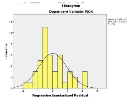
Gambar 2. Histogram
