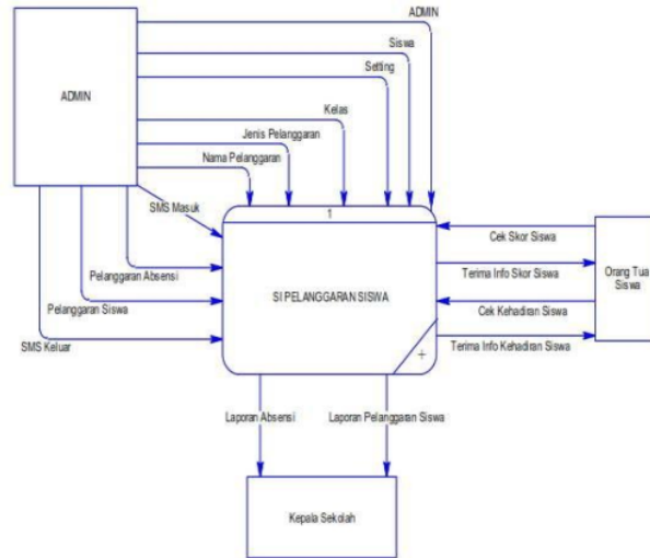
Gambar 1. Context Diagram
