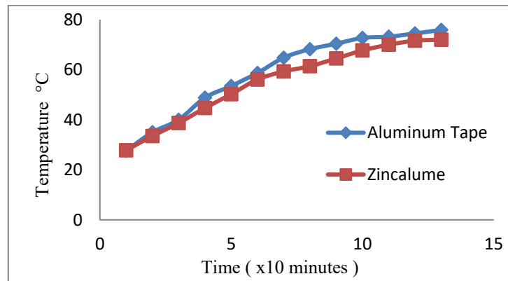
Figure 3. comparative perform of two reflector, aluminum tape and zinalume.
