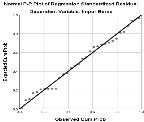
Gambar 3. Normalitas Probability Plot
